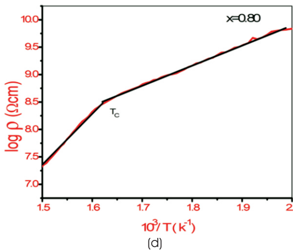
Figure 4. Graph of Log \rho Against (1000/T) for Mg_xZn_{1-x}Fe_2O_4 (a) ( x = 0.20 ); (b) ( x = 0.40 ); (c) ( x = 0.60 ); (d) ( x = 0.80 )
