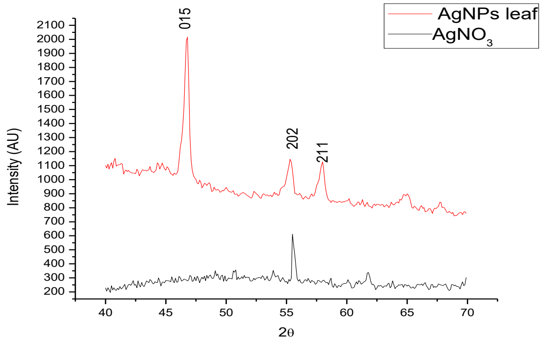
Fig. 4: XRD analysis of Standard AgNO 3 and Biosynthesized silver nanoparticles from leaf powder of Martynia annua Linn.
